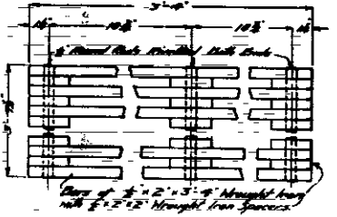
DETAIL OF GRATING SCALE 1/2" = 1'
